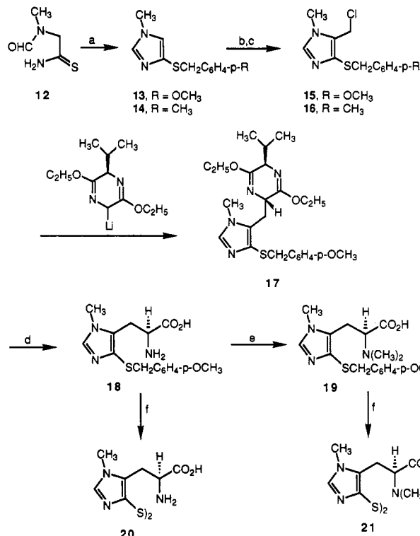
Scheme II a
